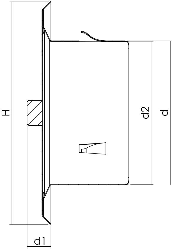
Side-intersection
