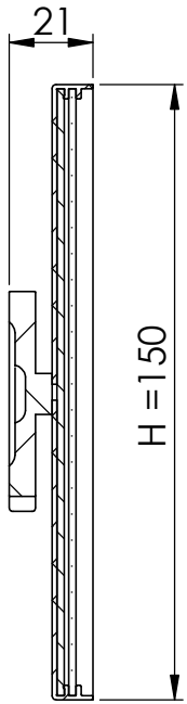
Side-intersection
