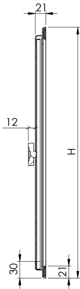
Side-intersection
